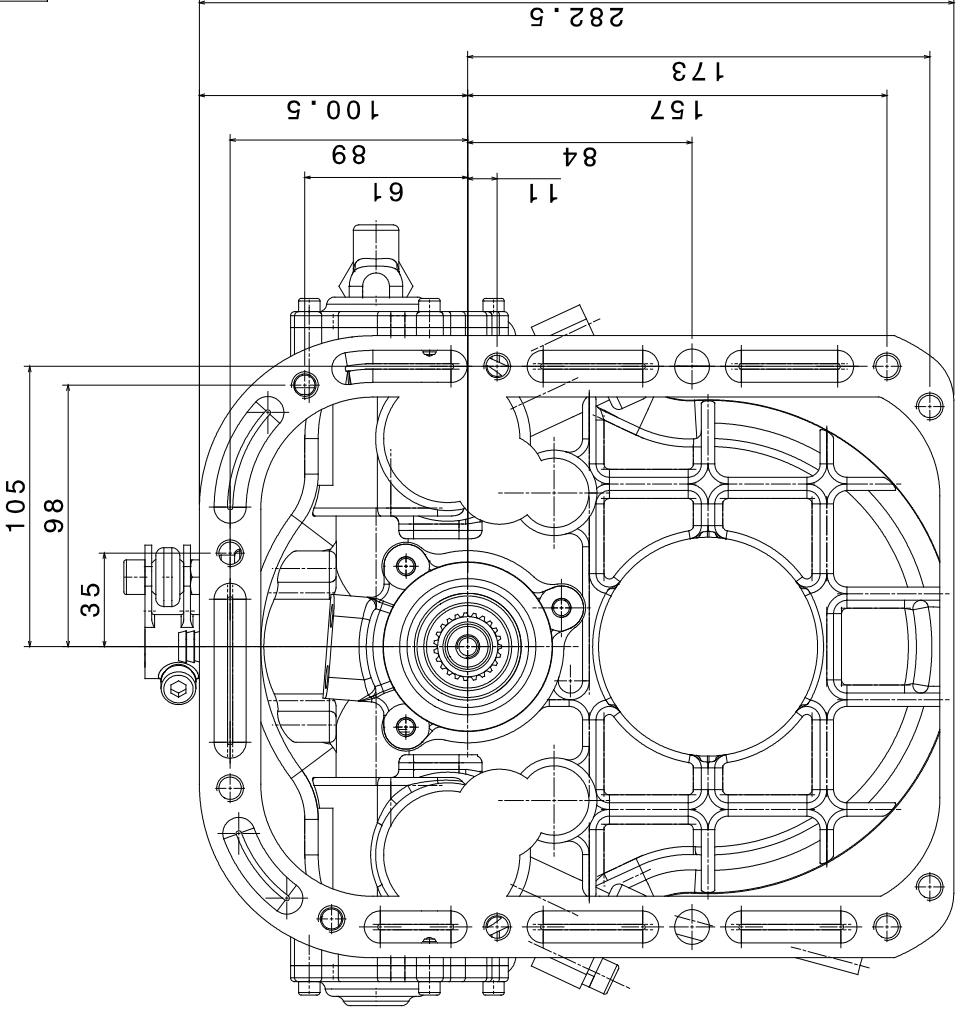
Gearbox SCL90 - 20
