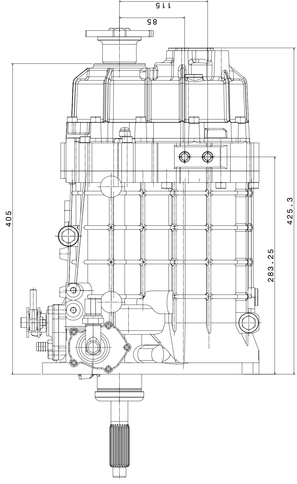
Gearbox SCL90 - 20
